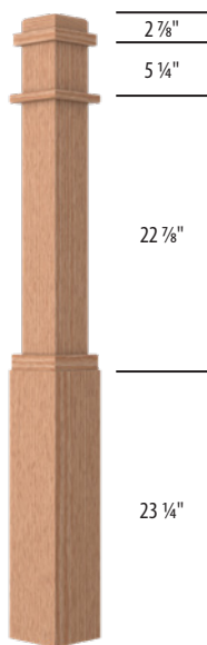
55 1/4" 5 1/2" LJ-4391CR Box Newel
