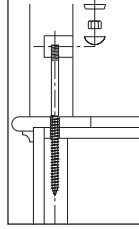
3008-10 NEWEL POST FASTENER 10-3/4"
